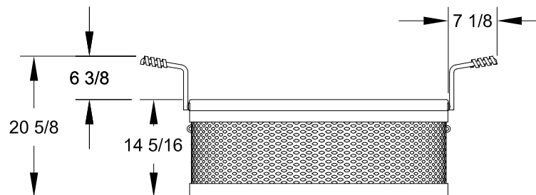
IAFS-30 ASSEMBLY
