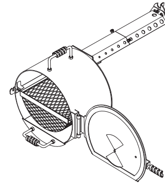
ECSFB-2640 Smoker for EC-26
