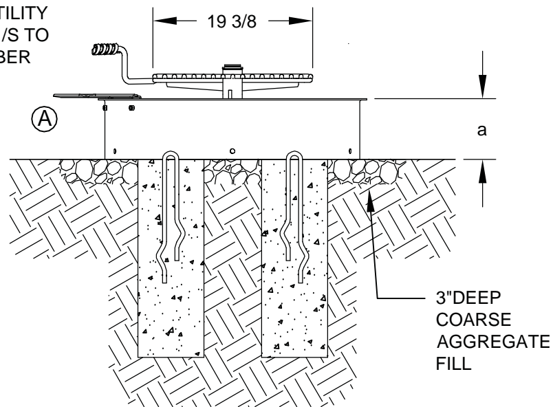
MODEL FSW-30/7/TB/S SHOWN WITH GRATE ROTATED
