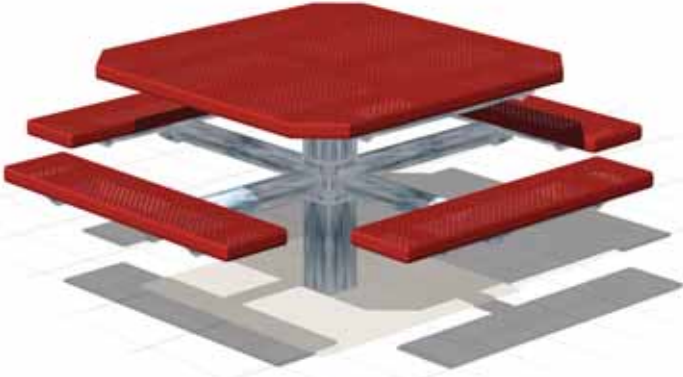
Model PQT/G-4VR 48" Square Top, Embedded Mount Table with hot dip galvanized frame and red V-Type thermo-plastic coated expanded steel top and seats
