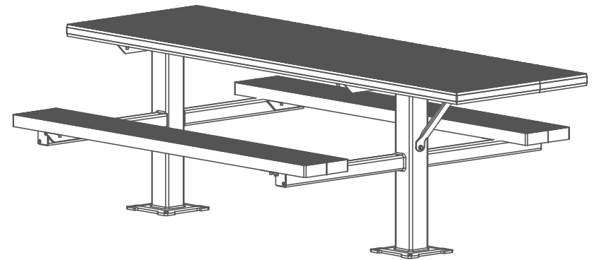
SHOWN WITH OPTIONAL 3/8" X 10" X 10" SURFACE MOUNT BASE PLATE WITH FOUR 25/32" DIA. HOLES
